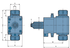
E37 Radial Double Drilling And Milling Heads
