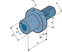
E55 Static Holders
