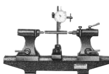
B82 Concentric Test Stand
