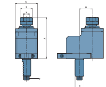
E40 Axial Drilling And Milling Heads
