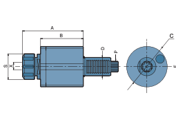
E38 Axial Drilling And Milling Heads
